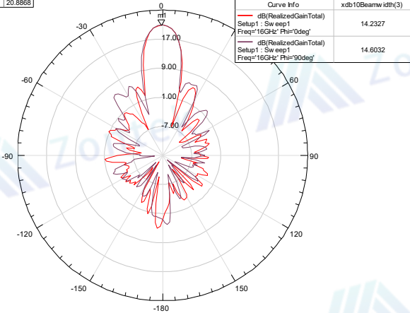
Radiation Pattern 15
