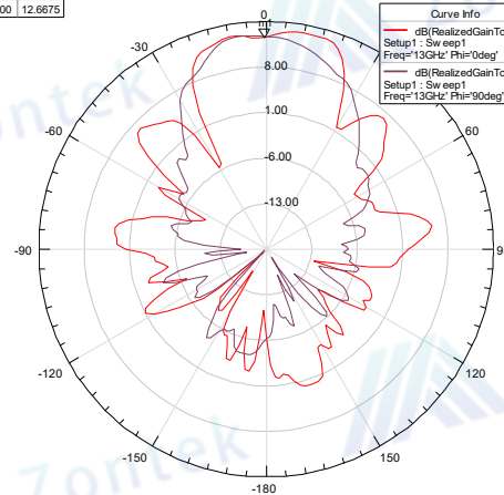
Radiation Pattern 12
