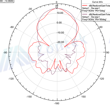
Radiation Pattern 8
