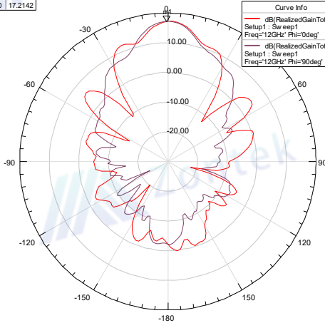
Radiation Pattern 11
