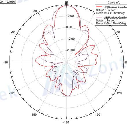
Radiation Pattern 10
