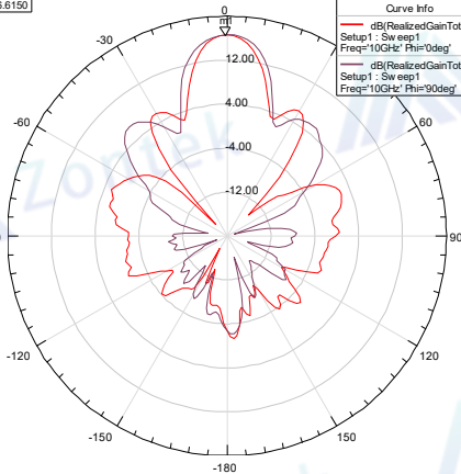
Radiation Pattern 9
