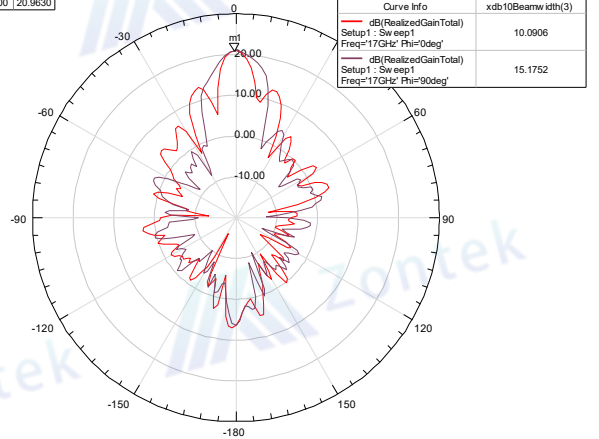
Radiation Pattern 16
