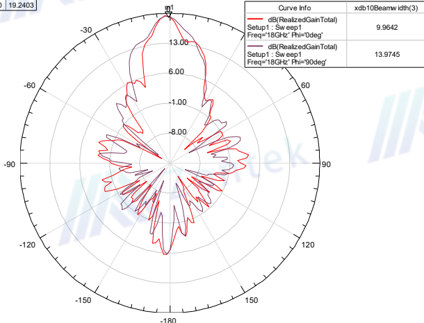
Radiation Pattern 17
