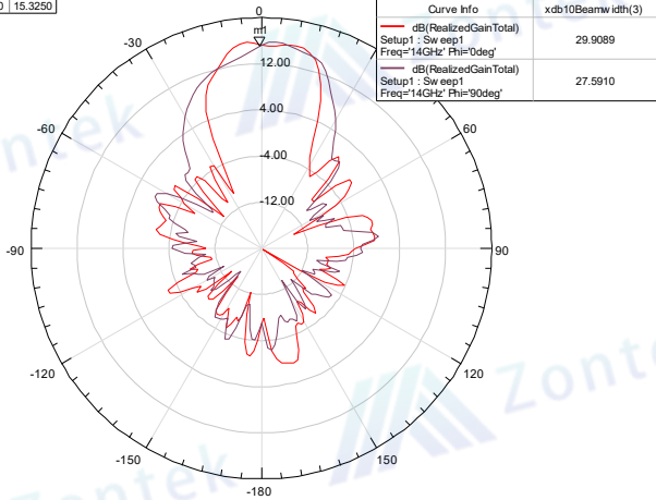
Radiation Pattern 13
