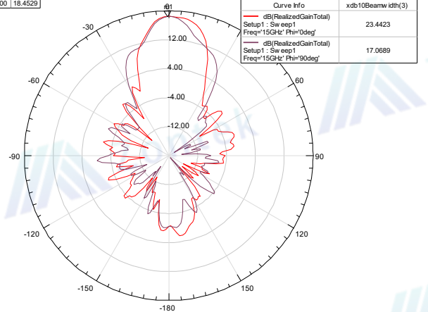
Radiation Pattern 14
