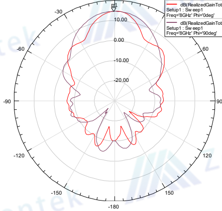
Radiation Pattern 7
